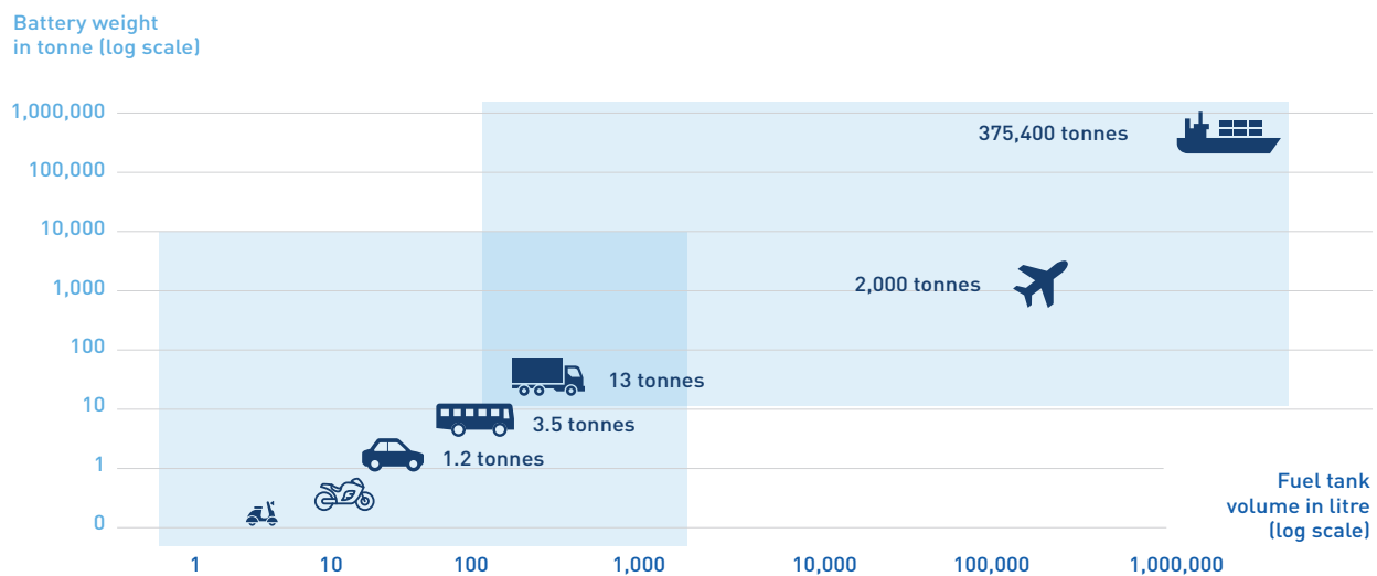
FIGURE 6: LIMITED ELECTRIFICATION BEYOND THE BUS AND LIGHT TRUCK SEGMENT
